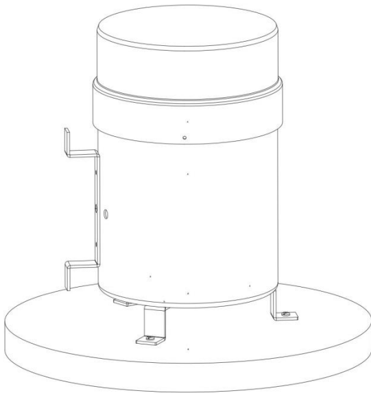
Model 525 Surface Mounted On a Masonry Block
